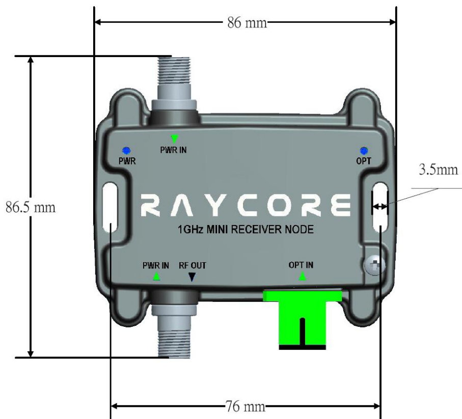
Product Drawing (unit: mm)
