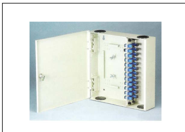
12C/24C ODF for Wall Mount
