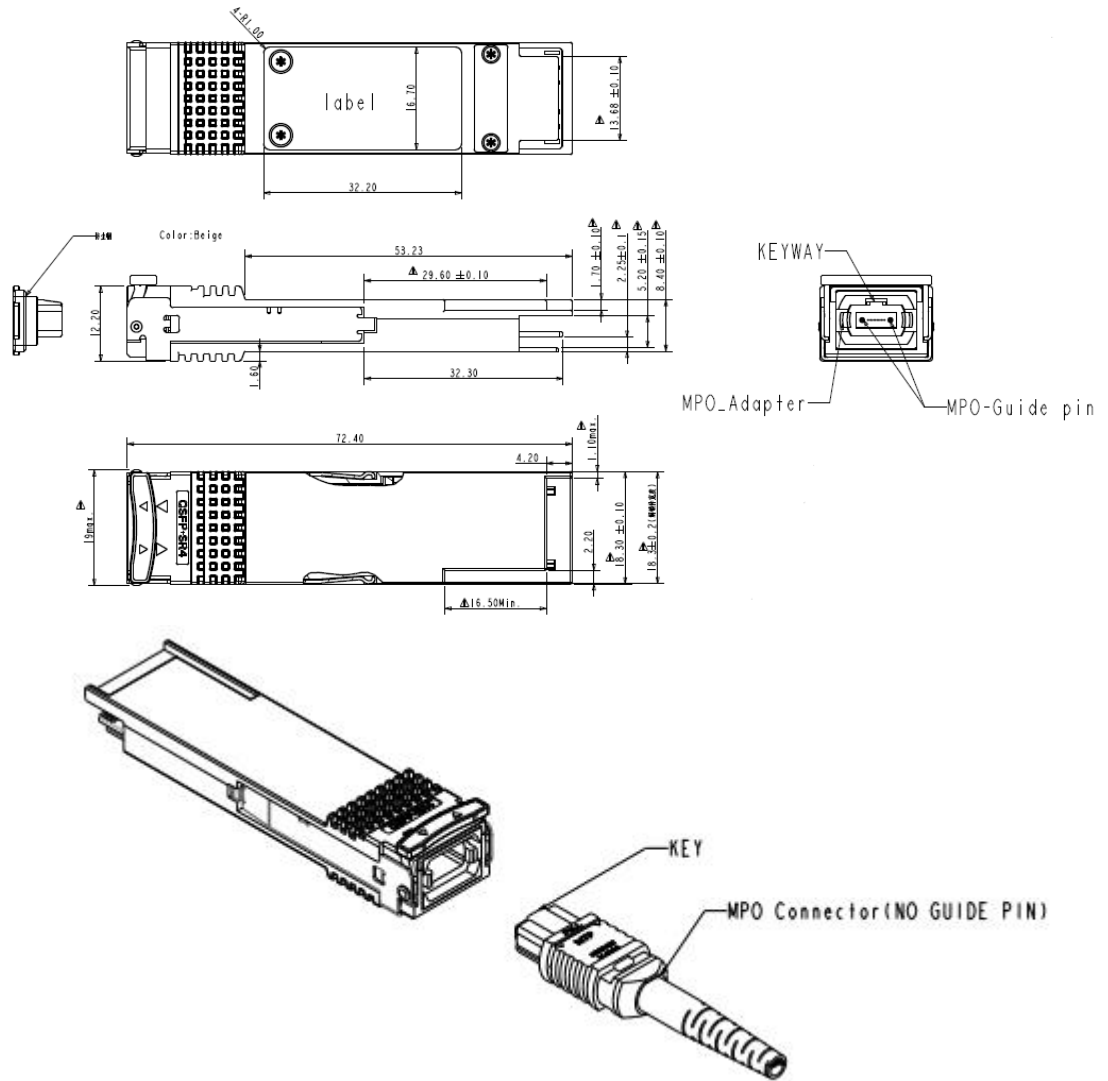
Figure10. Mechanical Specifications
