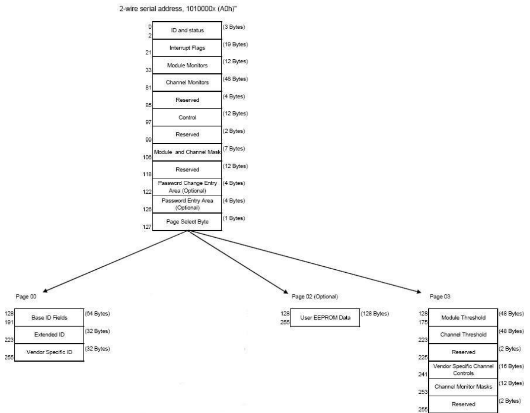
Figure5. QSFP Memory Map
