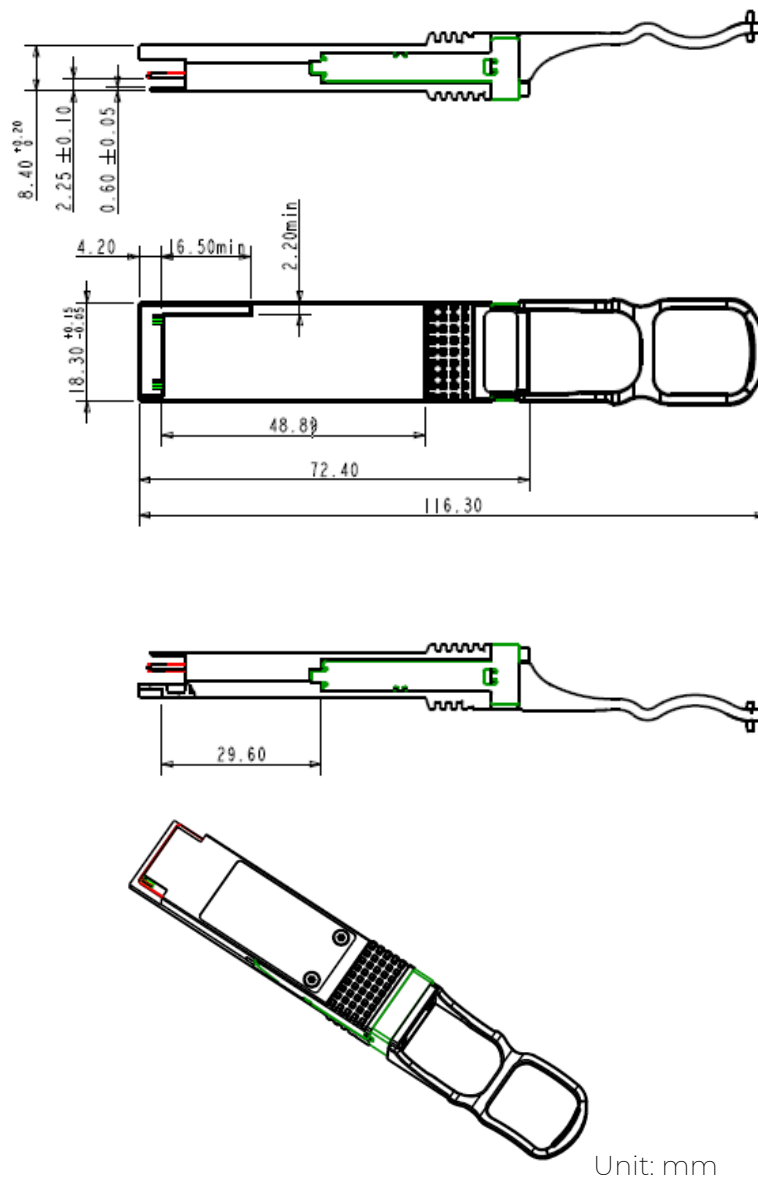
Figure10. Mechanical Specifications
